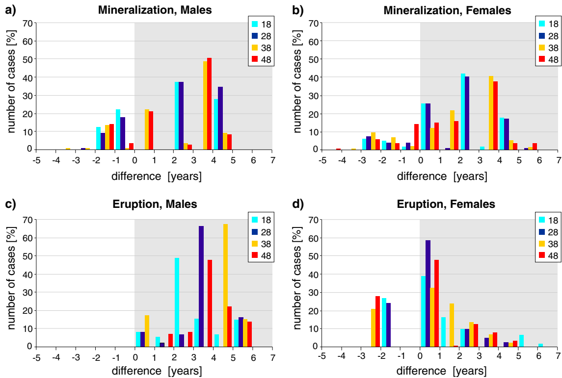
Fig. 1 Distribution of the estimation errors based on standard reference data on mineralization and eruption. The height of the columns represents the relative number of evaluated cases in percent with different colors for the individual wisdom teeth (18, 28, 38, 48); the x-axis shows the
