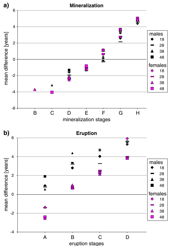
Fig. 3 Mean differences in years between estimated and chronological age corresponding to the different mineralization and eruption stages, respectively. Pink data points correspond to the values found for the different wisdom teeth in females, black data points stand for the values found in the males. For better visibility standard deviations are not shown
