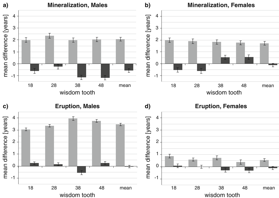
Fig. 4 Accuracy of estimations of dental age using standard reference values (light gray) and adjusted reference values (dark gray), respectively. The y-axis represents the mean difference between estimated dental age and chronological age in years. Error bars show the standard error of the mean
